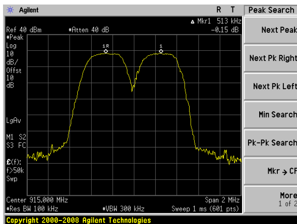
Channel Separation plot on channel 49-50
